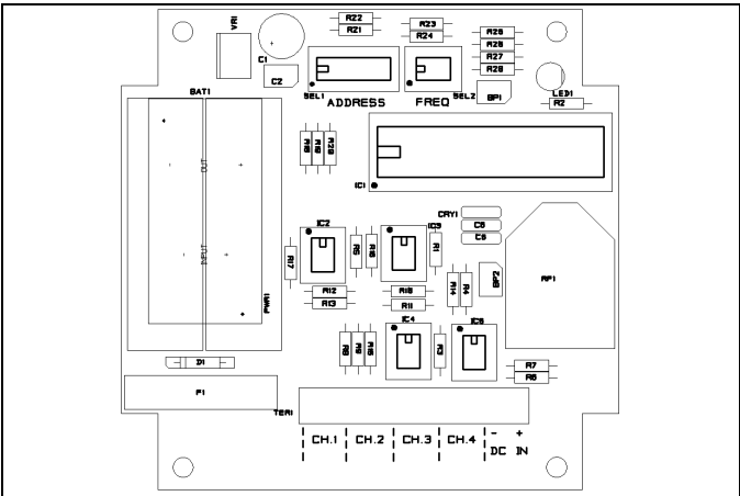
Wire as shown based on number of voltage inputs
